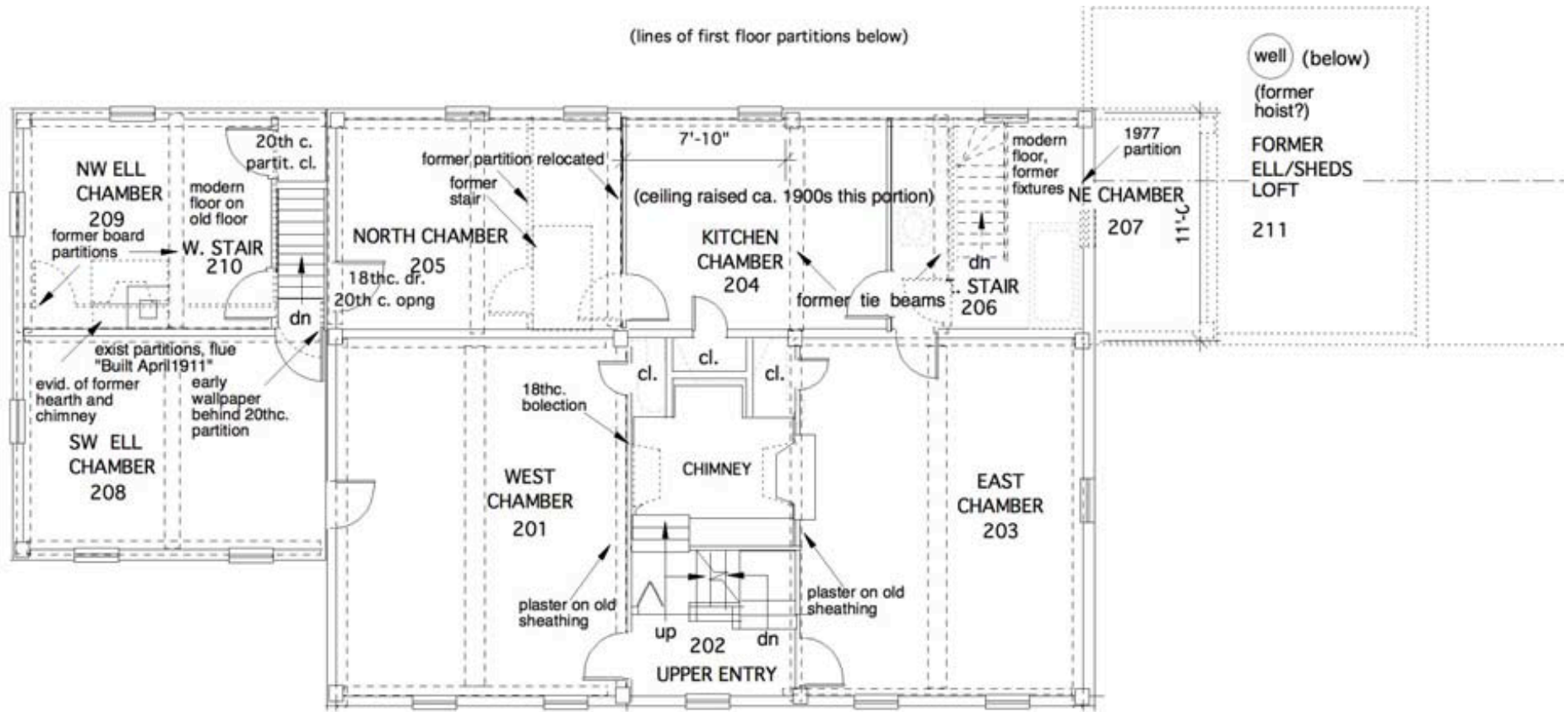
Second Floor Framing Plan
