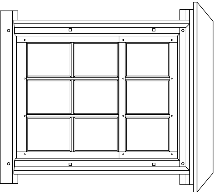
EXTERIOR ELEVATION TYPE D
